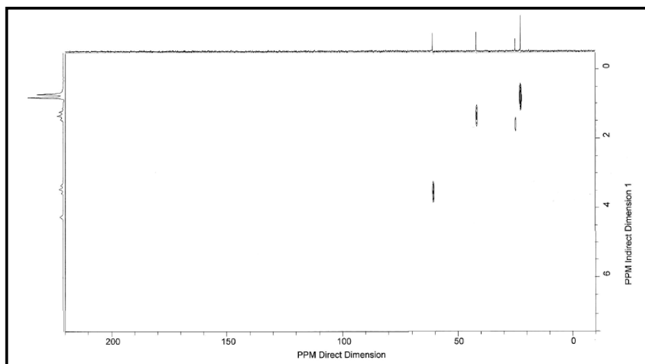
Figura 2 – Espectro 2D – HETECOR, ^1\text{H}/^{13}\text{C} de 1,3-diisobutóxiopropan-2-ol (DIBP) ( \text{CDCl}_3 – 60 MHz).
